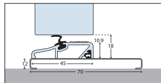
Standard open out ramped threshold
